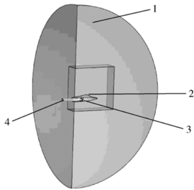
图 6 前机身/进气道一体化三维模型示意图 Fig. 6 Schematic structure of aeroplane forebody/air inlet integrated 3-D model
